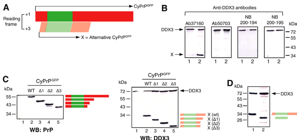
Figure 4. Translation of an overlapping ORF in the prion protein (PrP) CDS. A. Diagram of CyPrP GFP CDS (+1 reading frame) and frameshifted alternative CyPrP GFP (+3 reading frame). GFP CDS is shown in green, CyPrP CDS is shown in red. B. Western blot analysis of mock-transfected HEK293 cells (lane 1) and CyPrP GFP -transfected cells (lane 2) with four antibodies directed against DDX3, as indicated. DDX3 is indicated by an arrow above the 72 kDa marker. An unknown protein labeled X is detected in CyPrP GFP -expressing cells with antibodies Ab37160. C. Western blot analysis of different CyPrP GFP C-terminal deletion mutants with anti-PrP (left blot) or anti-DDX3 (right blot, Ab37160) antibodies. Lane 1: Mock-transfected cells; lane 2: cells transfected with wild-type CyPrP GFP ; lanes 3–5: deletion mutants. A diagram of each construct is indicated on the right side of each blot. C-terminal deletions within CyPrP GFP introduce C-terminal deletions within overlapping alternative CyPrP GFP . D. Western blot analysis of cells transfected with CyPrP GFP (lane 1) or frameshifted GFP (lane 2) with anti-DDX3 antibodies (Ab37160).
