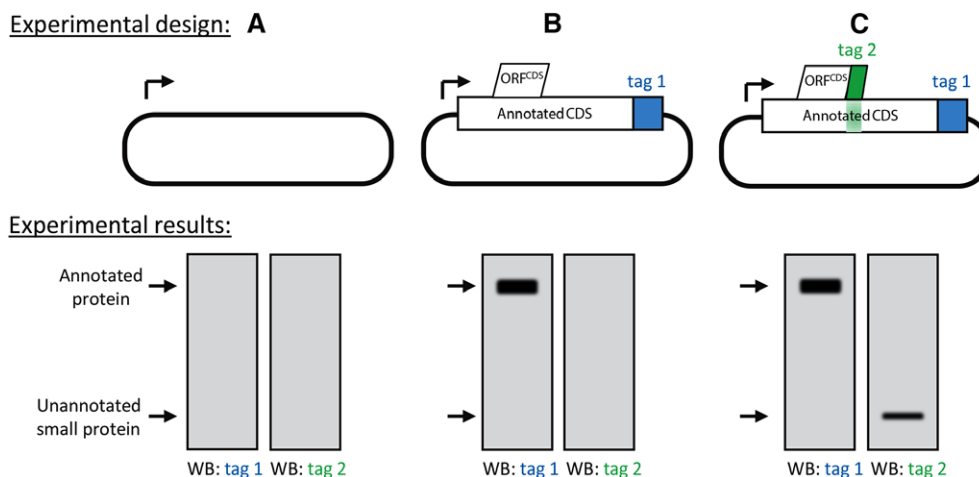
Figure 5. A simple double epitope tagging strategy for the detection of ORFs CDS . Upper panel: experimental design. (A) Empty vector. (B) Expression plasmid containing an epitope tagged CDS (tag1). (C) Expression plasmid containing both an epitope tagged CDS (tag 1) and an epitope tagged ORF CDS (tag 2). Tag 2 is in-frame with the ORF CDS , but out-of-frame with the CDS. Tag 2 should not introduce a stop codon in the CDS frame. Bottom panel: after transfection and expression, cell lysates are analyzed by western blot with anti-tag 1 and anti-tag 2 antibodies. (A) No signals are detected in mock-transfected cells. (B) Anti-tag 1 antibodies detect the expression of the protein of interest. A second protein expressed from the ORF CDS remain invisible. (C) Anti-tag 2 antibodies detect the expression of the unannotated small protein.
