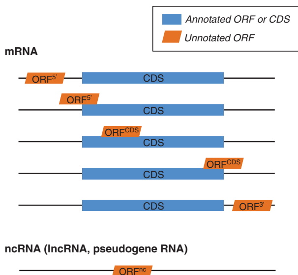
Figure 1. Unannotated ORFs may be found in mRNAs or non-coding RNAs. Molecules shown here represent mature or processed RNAs. Unannotated ORFs are found in untranslated regions of the transcriptome. Within mRNAs, these regions include 5'UTRs, 3'UTRs, and alternative reading frames overlapping annotated CDSs. An ORF 5' (also termed upstream ORF or uORF) may be found outside the CDS in the three reading frames, or partially overlapping a CDS in one of the two alternative reading frames. ORF CDS may be found completely nested inside the CDS, or partially overlapping the 3'UTR in one of the two alternative reading frames. An ORF 3' may be in one of the three reading frames. Non-coding RNAs do not have a tripartite structure similar to mRNAs, and an ORF nc may be found anywhere.
