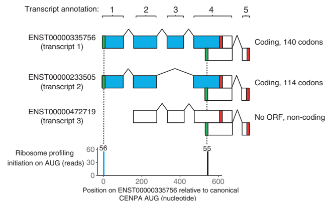
Figure 2. Typical Ensembl transcripts annotation for a human gene. Three transcripts from the CENPA gene are illustrated. Sequences annotated as coding sequences are shown as blue boxes, and sequences annotated as untranslated regions are shown as open boxes. Green boxes represent AUG translation initiation sites. Red boxes represent stop codons. ENST00000335756 carries the canonical 420 bps CDS with four coding exons. The end of exon 4 after the stop codon is non-coding. ENST00000233505 is an isoform lacking exon 3 and carries a shorter version of the canonical CDS. ENST00000472719 is an isoform lacking exon 1. In the absence of the translation initiation site, the Ensembl annotation indicates the absence of a canonical CDS, and this transcript is believed to be non-coding. An unannotated overlapping long ORF of 53 codons in the +2 reading frame starts with an AUG codon within exon 4 and ends with a stop codon in exon 5. Translation initiation ribosome profiling data clearly show initiating ribosomes on both the annotated CDS and the unannotated ORF with similar number of reads (graph below). Thus, transcripts 1 and 2 might be bicistronic, and transcript 3 is likely a coding transcript for a novel small protein.
