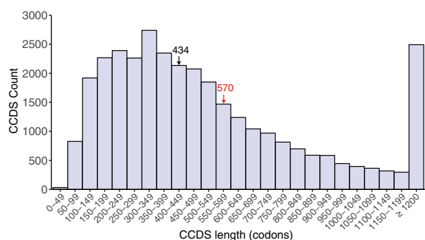
Figure 3. Distribution of the number and the size of human consensus CDSs. Calculations were performed with consensus CDS release 20. Median, 434 codons; average, 570 codons.
